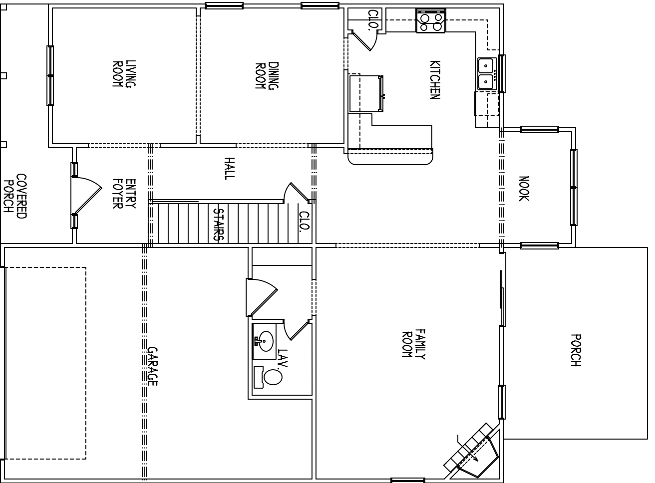
PROPOSED FIRST FLOOR LAYOUT PLAN
